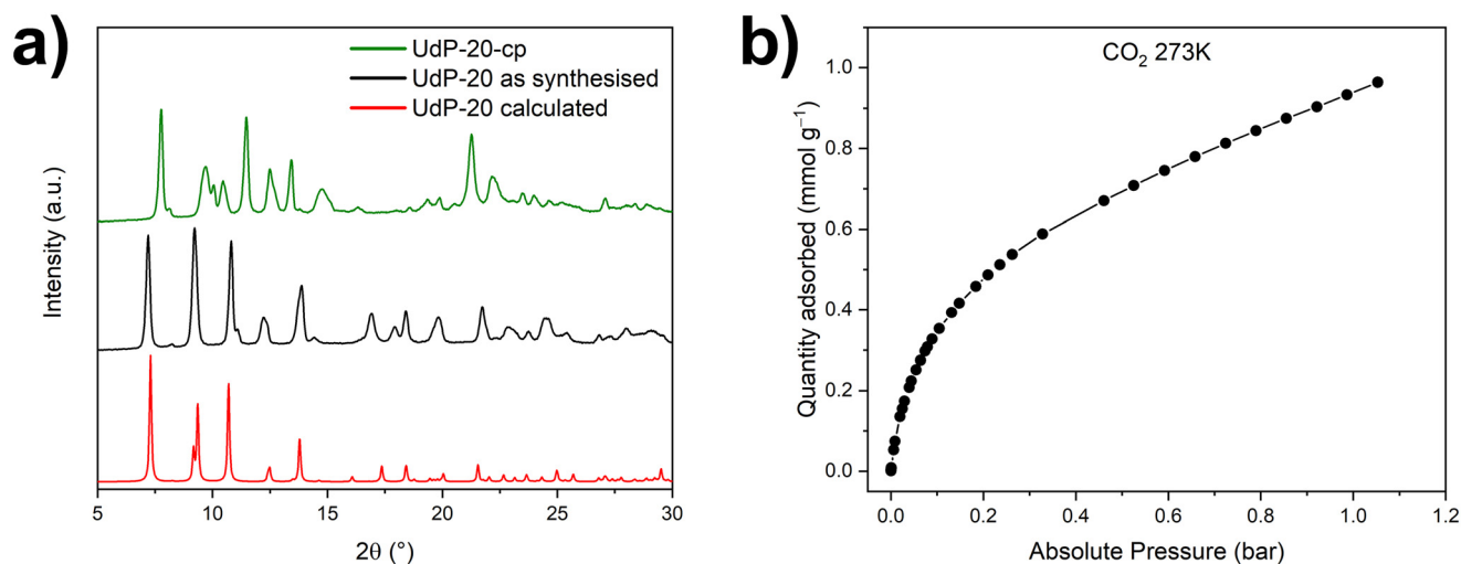
Fig. 3 PXRD pattern comparison between UdP-20 calculated (red), UdP-20 as synthesised and UdP-20 after the activation process (UdP-20-cp, green) (a). \text{CO}_2 isotherm at 273 K registered on UdP-20-cp. (b).
