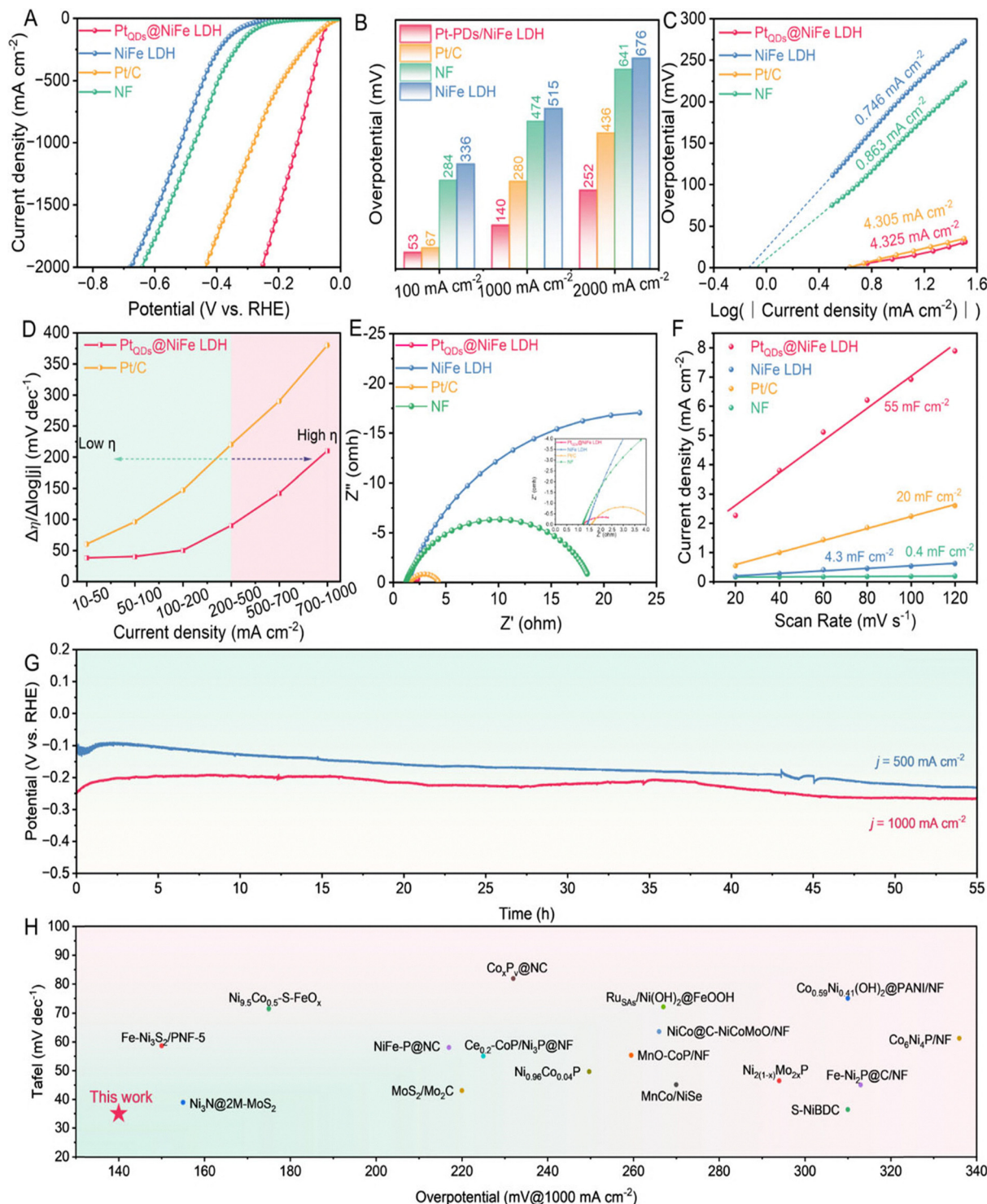
Fig. 10 HER curves (A) LSV plots; (B) plot of overpotential vs. log (current density); (C) j_0 of PtQDs@NiFe LDH some control samples are derived by Tafel plots; (D) Plot of \Delta\eta/\Delta\log|j| versus current density ranges; (E) comparative Nyquist plots; (F) plot of current density vs. scan rate; (G) potential vs. time plots; (H) plot of Tafel value vs. overpotential of PtQDs@NiFe LDH over other catalysts (reproduced with permission from ref. 61©OAE publishing, Inc.; License: CC-BY 4.0).
