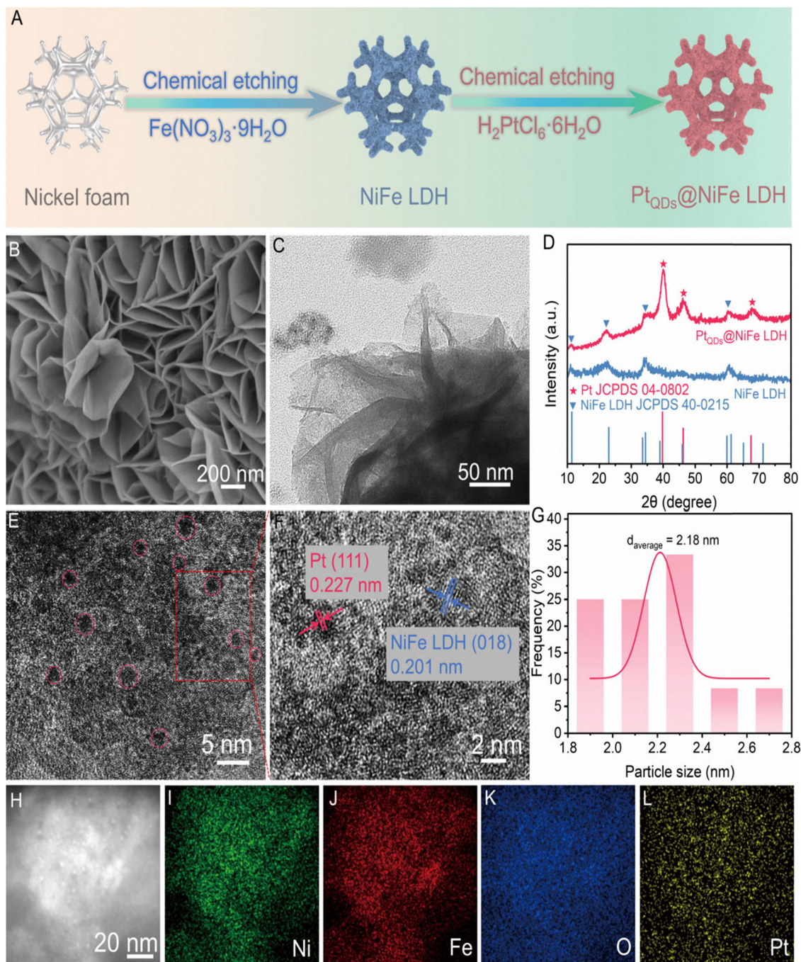
Fig. 9 (A) Schematic illustration of the synthesis of \text{Pt}_{\text{QDs}}@\text{NiFe LDH} , (B) and (C) SEM and HR-TEM images of \text{Pt}_{\text{QDs}}@\text{NiFe LDH} ; (D) XRD pattern of \text{Pt}_{\text{QDs}}@\text{NiFe LDH} and NiFe LDH; (E) and (F) HRTEM images of \text{Pt}_{\text{QDs}}@\text{NiFe LDH} ; (G) average particle size distribution of \text{Pt}_{\text{QDs}} ; (H)–(L) EDX mapping patterns of various elements within \text{Pt}_{\text{QDs}}@\text{NiFe LDH} (reproduced with permission from ref. 61©OAE publishing, Inc.; License: CC-BY 4.0).
