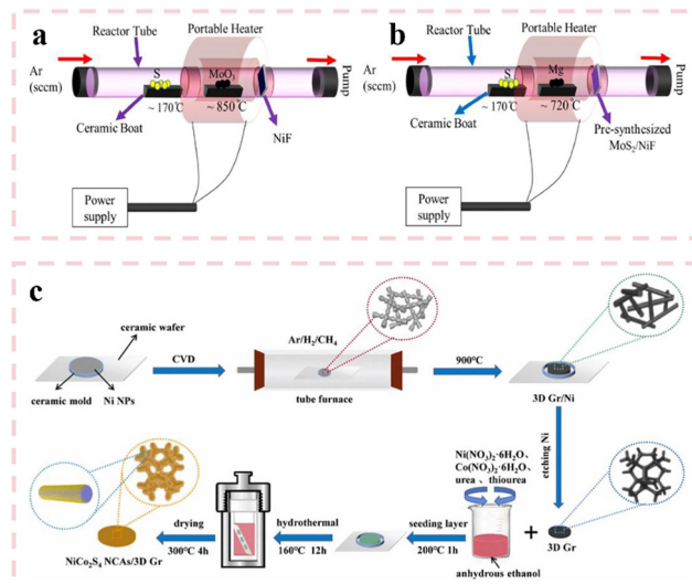
Fig. 5 Schematic diagram for the synthesis of (a) \text{MoS}_2 and (b) \text{MgS}/\text{MoS}_2 @ \text{NiF} EMS. Reproduced with permission from ref. 80. (c) Schematic of the preparation process of \text{NiCo}_2\text{S}_4 NCAs/3D Gr. Reproduced with permission from ref. 81.
