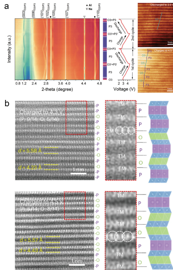
Fig. 7 (a) In situ XRD and corresponding STEM-HAADF images of the \text{Na}_{2/3}\text{Li}_{1/6}\text{Fe}_{1/6}\text{Co}_{1/6}\text{Ni}_{1/3}\text{Mn}_{1/3}\text{O}_2 cathode when charging to 4.5 V and discharging to 2.0 V, respectively. Reproduced with permission from ref. 80, copyright 2022 Wiley. (b) STEM-HAADF images of the \text{Na}_{0.67}\text{Li}_{0.1}\text{Fe}_{0.37}\text{Mn}_{0.53}\text{O}_2 cathode at 4.3 V and 4.5 V charging states, respectively. Reproduced with permission from ref. 81, copyright 2024 Springer Nature.
