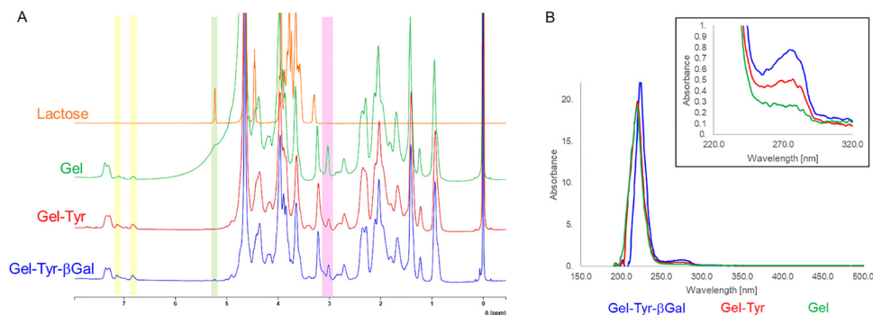
Fig. 2 1 H-NMR spectra of Gel-Tyr-βGal, Gel-Tyr, Gel, and Lactose with highlighted main peaks (A), and UV-VIS graphs of Gel-Tyr-βGal, Gel-Tyr, and Gel with a magnified view of the tyramine peak region (B). In this case, Gel-Tyr-βGal exhibits an even higher peak than Gel-Tyr, confirming that sugar conjugation does not impact the success of tyramine grafting.
