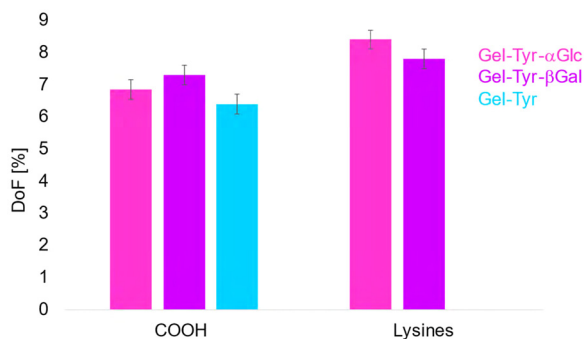
Fig. 3 Graph representing the molar DoF of lysines and carboxylic groups in Gel-Tyr-αGlc, Gel-Tyr-βGal and Gel-Tyr.
