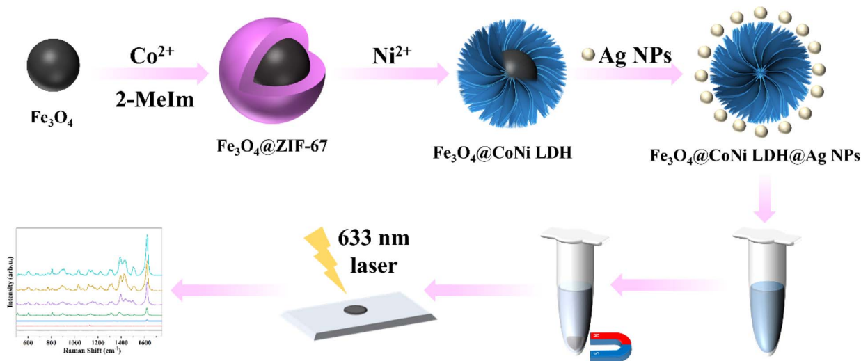
Scheme 1 Schematic of the preparation of the \text{Fe}_3\text{O}_4@\text{CoNi LDH}@Ag\text{ NP} SERS substrate and the process used for SERS detection.
