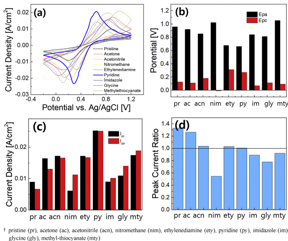
† pristine (pr), acetone (ac), acetonitrile (acn), nitromethane (nim), ethylenediamine (ety), pyridine (py), imidazole (im), glycine (gly), methyl-thiocyanate (mty) Fig. 8 Electrochemical performance comparison of Fe(II) complexing ligands by CV measurements for 20 cycles at a scan rate of 30 mV s -1 : (a) CV curves (the average), (b) anodic and cathodic peak potentials ( E_{pa} , E_{pc} ), (c) anodic and cathodic peak currents ( I_{pa} , I_{pc} ), and (d) peak current ratio [reproduced with permission 66 ].
