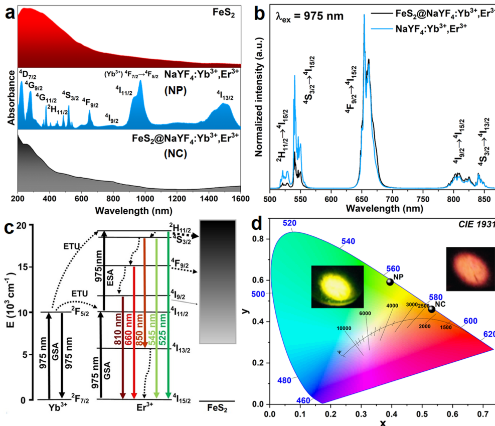
Fig. 3 Absorption spectra of the \text{FeS}_2 NPs (red), \text{NaYF}_4:\text{Yb}^{3+},\text{Er}^{3+} NPs (blue), and \text{FeS}_2@\text{NaYF}_4:\text{Yb}^{3+},\text{Er}^{3+} NC (black) (a). Normalized UC luminescence emission spectra of the \text{NaYF}_4:\text{Yb}^{3+},\text{Er}^{3+} NPs (blue), and the \text{FeS}_2@\text{NaYF}_4:\text{Yb}^{3+},\text{Er}^{3+} NC (black) under 975 nm laser excitation (b); energy level scheme of UC luminescence for the \text{FeS}_2@\text{NaYF}_4:\text{Yb}^{3+},\text{Er}^{3+} material (c); CIE diagram of the \text{NaYF}_4:\text{Yb}^{3+},\text{Er}^{3+} NPs and \text{FeS}_2@\text{NaYF}_4:\text{Yb}^{3+},\text{Er}^{3+} NC luminescence (d); insets show the visible luminescence of the \text{NaYF}_4:\text{Yb}^{3+},\text{Er}^{3+} NPs (yellowish-green) and \text{FeS}_2@\text{NaYF}_4:\text{Yb}^{3+},\text{Er}^{3+} NC (orange) taken with a digital camera upon laser excitation.
