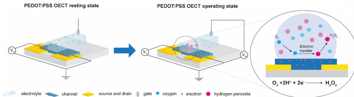
Fig. 1 A schematic of PEDOT:PSS OECT in its resting state and upon V_g operation, showing electron transfer from the polymer channel to the electrolyte and consequent generation of \text{H}_2\text{O}_2 .
