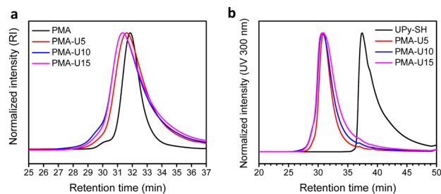
Fig. 4 SEC traces of the purified PMA-UPy polymers. (a) RI signal; (b) UV signal at 300 nm.
