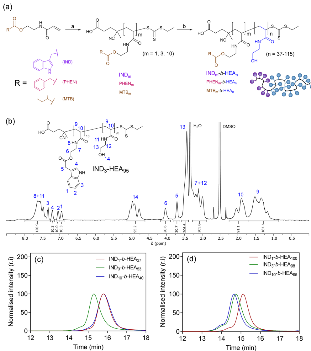
Fig. 3 (a) Synthesis of IND_m^- , PHEN_m^- , MTB_m^-b-HEA_n block copolymers. Reagents and conditions: (a) AIBN, CTA, DMF, 80 °C; (b) N -hydroxyethyl acrylamide, V501, DMF, 70 °C; (c) ^1H NMR (DMSO- d_6 , 400 MHz) spectrum of IND_3-b-HEA_{95} as a representative spectrum of the synthesised block copolymers; SEC chromatograms of IND_m-b-HEA_n copolymers with (c) shorter and (d) longer hydrophilic blocks, using DMF with 0.1% LiBr as the mobile phase. Spectra and SEC chromatograms of all polymers are shown in Sections S5.3.1 and S5.3.2 in the ESI.†
