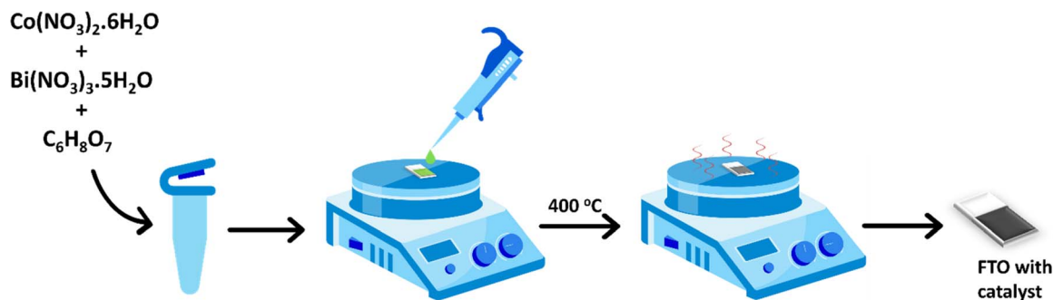
Fig. 1 Schematic of the synthesis of \text{Co}_3\text{Bi}_x\text{O}_x catalysts on FTO. The procedure involves: (i) mixing \text{Co(II)} nitrate and \text{Bi(III)} nitrate in citric acid solution, (ii) deposition of the solution onto FTO substrate, and (iii) drying and annealing the FTO-deposited metal salts.
