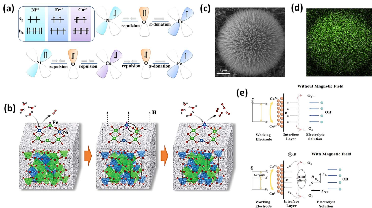
Fig. 18 (a) Schematic of the electronic interaction in the d_{xy} orbitals of \text{NiFe-LDH} and \text{Cu-NiFe-LDH} (reprinted with permission, 195 copyright 2022, the American Chemical Society). (b) Schematic showing the increase in concentration of \text{Ni}^{3+} at the T_d sites (reprinted with permission, 196 copyright 2022, Wiley). (c) and (d) SEM image and elemental mapping of \text{Co}_3\text{O}_4 , respectively, and (e) mechanistic illustration of magnetic field-enhanced OER activity of \text{Co}_3\text{O}_4 (reprinted with permission, 197 copyright 2019, Elsevier).
