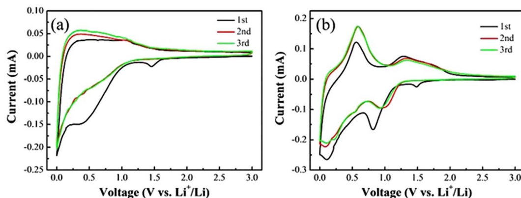
Fig. 5 Cyclic voltammety plots for the first three cycles of (a) carbon fibre anodes and (b) a CFBA consisting of \text{SnO}_2 coated carbon fibres. 25 Reproduced from ref. 25 with permission from Elsevier, copyright 2024.
