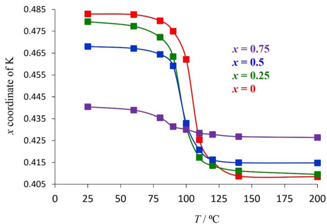
Fig. 9 The temperature dependence of the potassium coordinate ( x , x ) in as-prepared K_{1-x}Cs_xTa_{0.5}Nb_{0.5}WO_6 ( 0 \leq x \leq 0.75 ), determined from Rietveld analysis of synchrotron powder X-ray diffraction data collected at temperatures in the range 25 \leq T/^\circ C \leq 200 . The error bars lie within the points.
