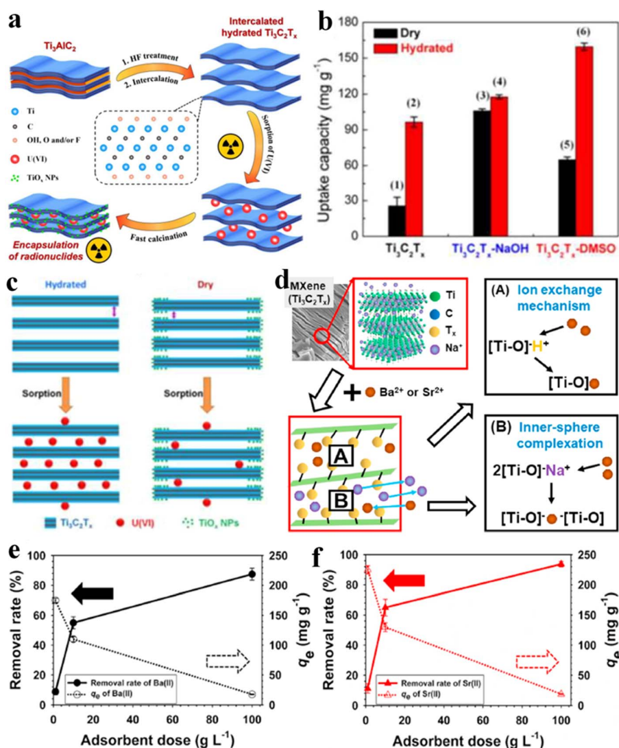
Fig. 22 (a) Synthesis of Ti_3C_2T_x via a hydrated-intercalation approach. (b) Comparative performances obtained for Ti_3C_2T_x , Ti_3C_2T_x-NaOH , and Ti_3C_2T_x-DMSO . (c) Sorption of U(VI) on hydrated and dry MXenes, reproduced from ref. 361 with permission from Royal Society of Chemistry, copyright 2017. (d) Adsorption of Ba/Sr via MXene. (e) Percentage removal and q_e ( mg\ g^{-1} ) of Ba and (f) percentage removal and q_e ( mg\ g^{-1} ) of Sr by increasing the dose of MXene ( g\ L^{-1} ), reproduced from ref. 362 with permission from Elsevier, copyright 2020.
