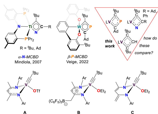
Fig. 1 Top: Isolable pnictogen-based metallacyclobutadienes (MCBD) complexes and the vanadacyclobutadiene (VCBD) species reported in this work ( L = dBDI^{2-} ). Bottom: Selected [V^V] alkyldiene complexes, with complex C being the focus of the present study.
