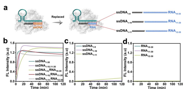
Fig. 2 Detection of RNA substrates using split activators in the CRISPR/Cas12a system. (a) Schematic representation of the CRISPR/Cas12a system activated by inputting replaced RNA. Real-time fluorescence of the Cas12a/crRNA complex binding to different activators (b) fragmented ssDNA and RNA (total 30 nt); (c) ssDNA (9–11 nt); (d) RNA (19–21 nt).
