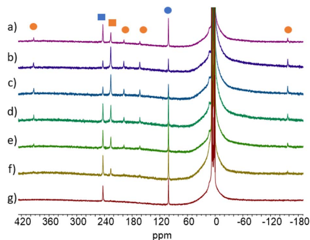
Fig. 6 ^1\text{H} NMR of 2-Tb at different PSS (after 30 min of irradiation) depending on the wavelength of the irradiation light used (a) t = 0 , (b) \lambda = 370 nm, (c) \lambda = 390 nm, (d) \lambda = 427 nm, (e) \lambda = 467 nm, (f) \lambda = 490 nm, (g) \lambda = 525 nm. Blue is for 2- cis and orange for 2- trans . Squares are for the Cot ligand, and circles are for the Cnt ligand.
