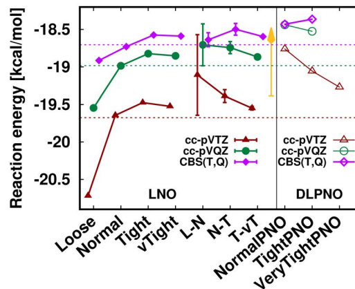
Fig. 5 Reaction energy of octamethylcyclobutane (OMCB) dimerized from 2,3-dimethylbut-2-ene of the NWH reaction compilation. 30 The plot shows LNO-CCSD(T) (left), LAF extrapolated LNO-CCSD(T) according to eqn (5) (middle) and DLPNO-CCSD(T 1 ) (right) results compared to the horizontal lines corresponding to the conventional CCSD(T) results. The Normal LNO-CCSD(T)/ \Delta CBS(T,Q) basis set correction to Normal - Tight LNO-CCSD(T)/haTZ in the composite E_{\text{LAF}}^{\text{CBS}(X+1),X} / \text{CCSD(T)} approach of eqn (7) is depicted as an orange vertical arrow.
