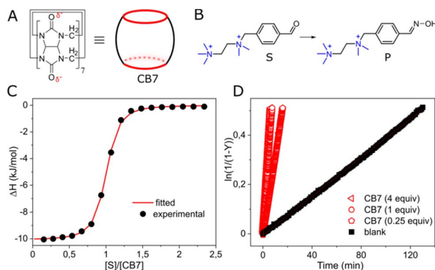
Fig. 1 (A) Chemical structure and cartoon representation of cucurbit[7]uril (CB7); (B) oxime formation reaction; (C) titration of CB7 with the substrate, water, pH = 6 (adjusted with HCl/NaOH), 298 K; (D) kinetic traces for the reaction progress at various amounts of CB7, [S] = 0.01 mM, water, pH = 6 (adjusted with HCl/NaOH), 298 K.
