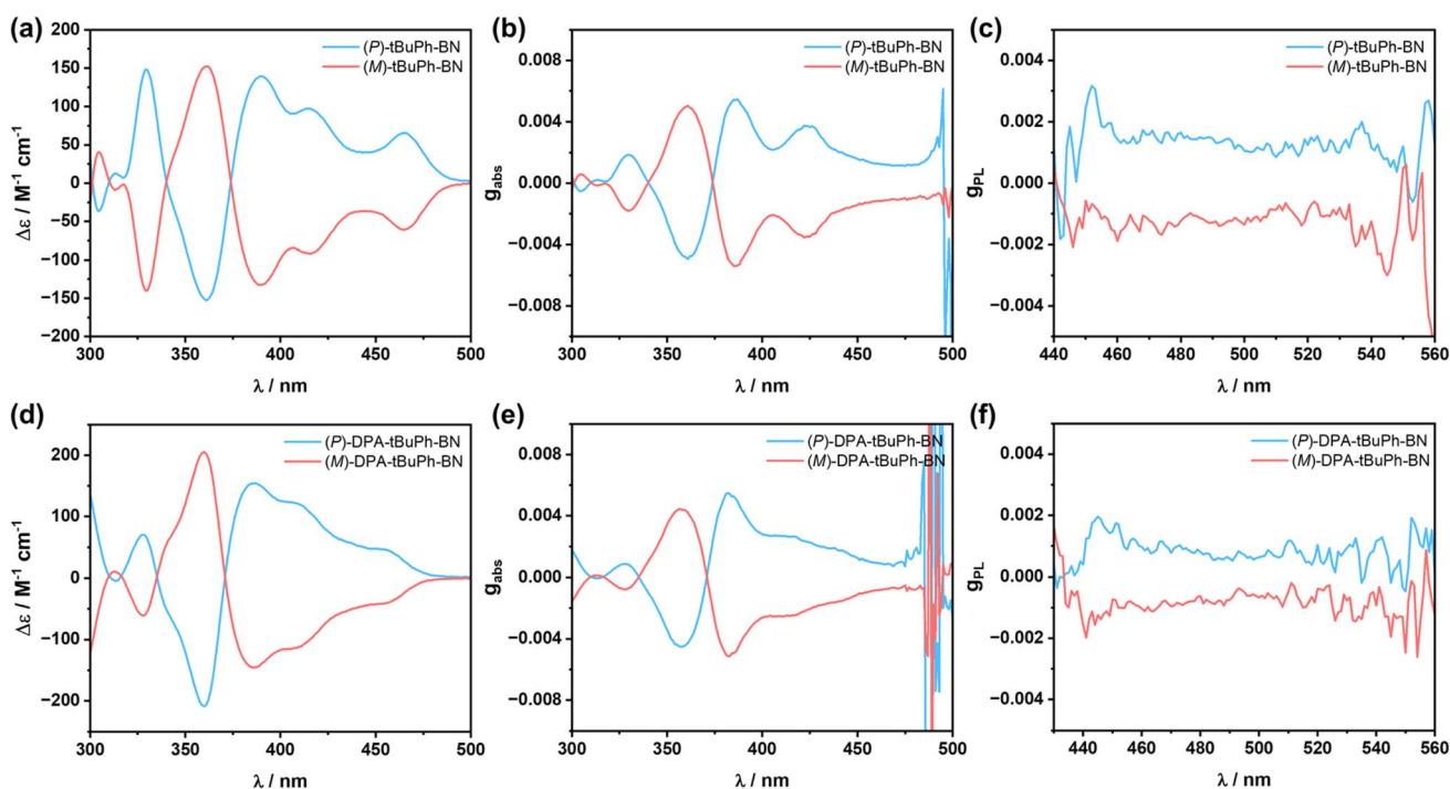
Fig. 6 (a) CD spectra and (b) g_{\text{abs}} values of tBuPh-BN recorded in 5 \times 10^{-6} \text{ mol L}^{-1} toluene solution. (c) g_{\text{PL}} values of tBuPh-BN recorded in 10^{-5} \text{ mol L}^{-1} THF solution. (d) CD spectra and (e) g_{\text{abs}} values of DPA-tBuPh-BN recorded in 5 \times 10^{-6} \text{ mol L}^{-1} toluene solution. (f) g_{\text{PL}} values of DPA-tBuPh-BN recorded in 10^{-5} \text{ mol L}^{-1} THF solution.
