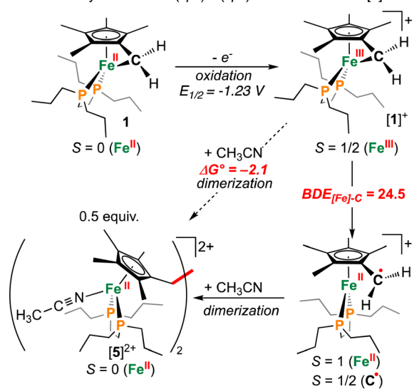
B. Thermodynamics for ethane elimination in [2]^+ (not observed)
