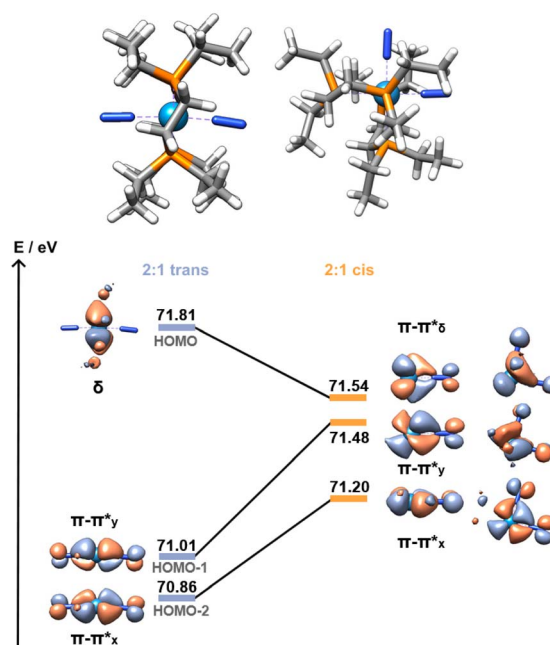
Fig. 7 Cis ( 11_{\text{Al}} ) vs. trans ( 8_{\text{Al}} ) frontier orbitals (HOMO to HOMO–2). AICF omitted for clarity. Orbitals of the cis isomer are shown in side and top views.
