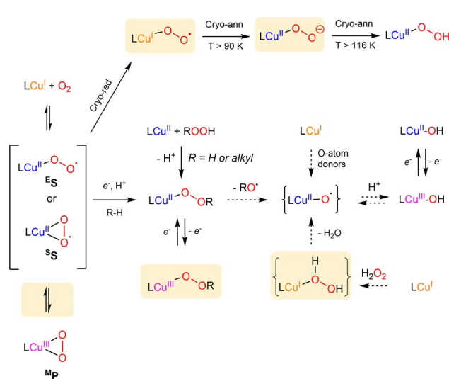
Scheme 5 Summary of known formation and interconversion pathways of mononuclear copper-oxygen entities. Recently isolated species or pathways are highlighted in orange. Dotted arrows correspond to postulated conversions pathways. The nomenclature used is derived from Stack et al. 2
