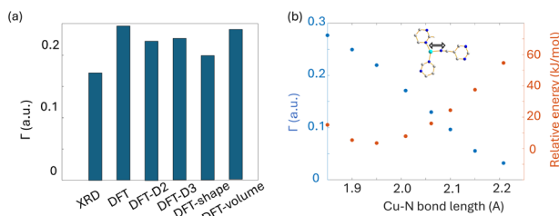
Fig. 9 (a) The EFG distance of optimized \text{Cu}_3(4\text{hypymca})_3 structure with different approaches, along with (b) the dependence of I on Cu-N bond length.
