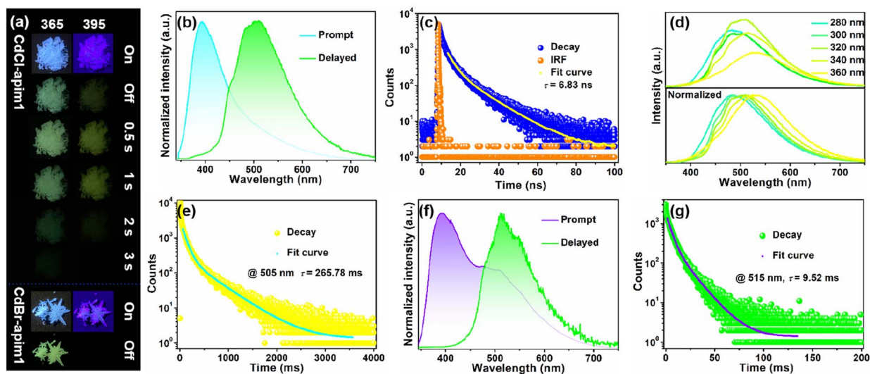
Fig. 3 (a) Photographs of \text{CdCl-apim1} and \text{CdBr-apim1} before and after removing the 365/395 nm UV lamp; the prompt and delayed spectra of \text{CdCl-apim1} (b) and \text{CdBr-apim1} (f); (c) fluorescence decay profile of \text{CdCl-apim1} ; (d) delayed spectra of \text{CdCl-apim1} excited by different wavelengths; phosphorescence decay profiles of \text{CdCl-apim1} (e) and \text{CdBr-apim1} (g).
