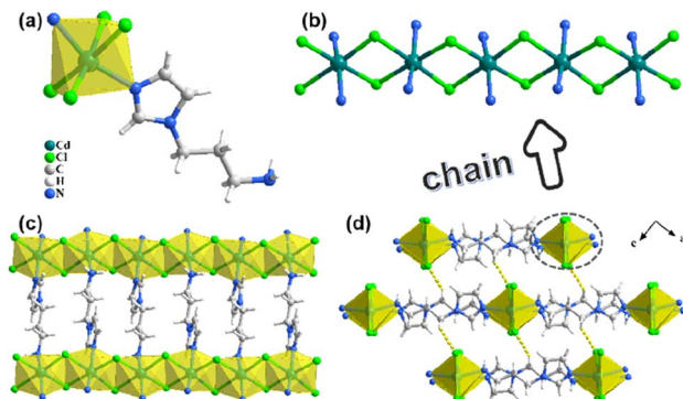
Fig. 2 (a) The asymmetric unit of \text{CdCl-apim2} ; (b) 1D chain; (c) 2D layer; (d) 3D supramolecular structure along the b axis (yellow dashed lines: \text{C-H}\cdots\text{Cl} ).
