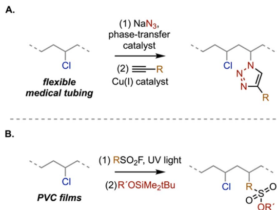
Scheme 3 Click reaction pathways for a two-step PVC functionalization, including an (A) azide-alkyne cycloaddition 90 and (B) SuFEx reactions. 91
