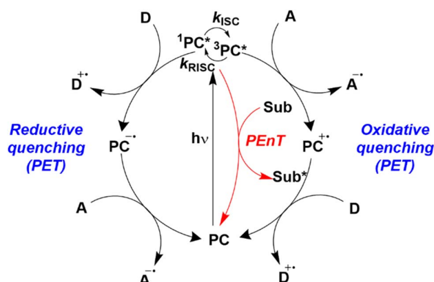
Fig. 1 Energy transfer, oxidative quenching, and reductive quenching photocatalytic cycles where D is an electron donor, A is an electron acceptor and Sub is a substrate. A and D can be reagents (substrates), reaction intermediates, other catalytic species, or sacrificial agents. Figure taken from ref. 5.
