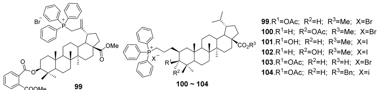
Fig. 31 The structures of BA derivatives 99 to 104.
