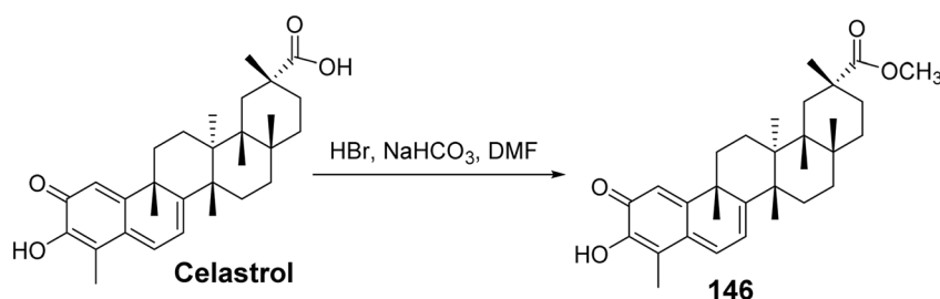
Fig. 43 Synthesis of celastrol derivative 146.
