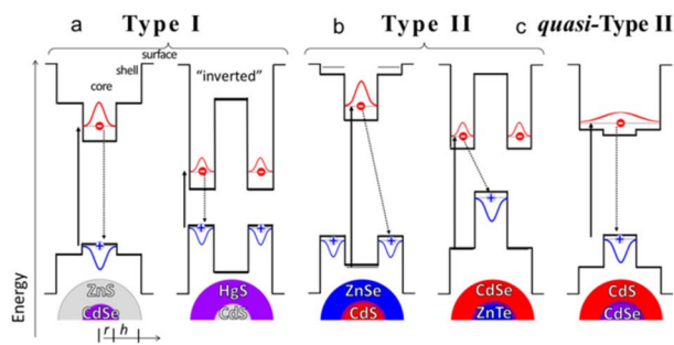
Fig. 1 (a) Type-I, (b) Type-II, and (c) quasi-Type-II band-edge alignments between the materials in core/shell QDs. Reprinted with permission from ref. 21 Copyright (2016) American Chemical Society.
