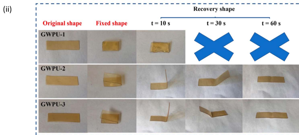
Fig. 8 (i) Reaction scheme of the synthetic route of the non-ionic GWPU dispersions and (ii) photographs of shape memory process of GWPU/GF polymers. Reprinted with permission. 36 Copyright 2022, Elsevier.
