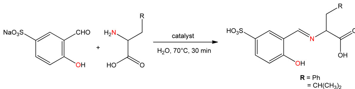
Fig. 9 Synthesis of water-soluble amino acid Schiff base ligand.
