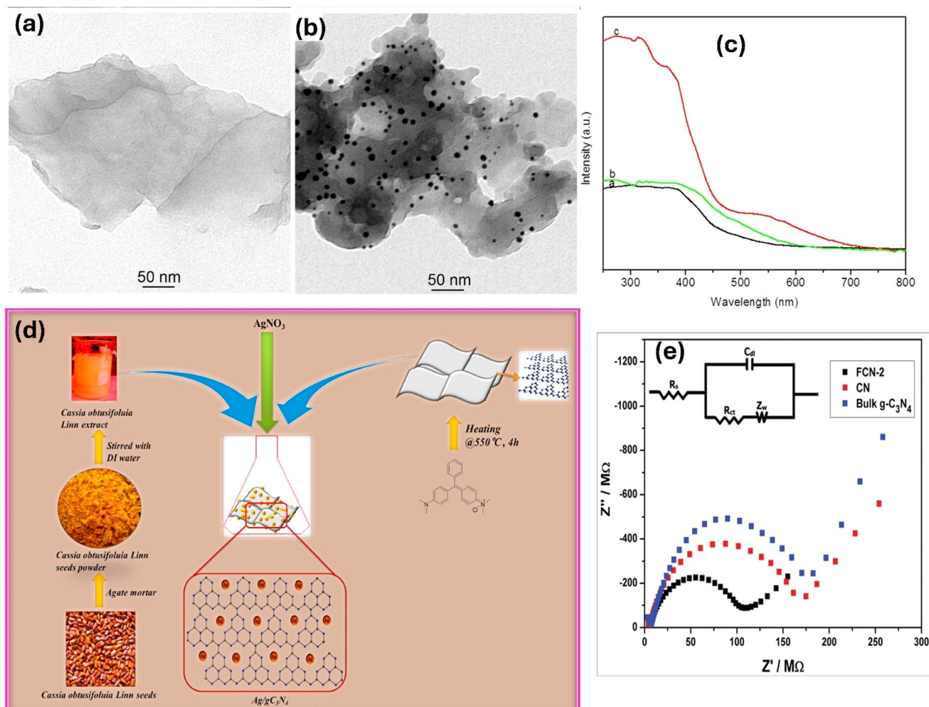
Fig. 2 Tem image of (a) \text{g-C}_3\text{N}_4 , (b) Au/ \text{g-C}_3\text{N}_4 , (c) DRS data of \text{g-C}_3\text{N}_4 nanosheets, bulk \text{g-C}_3\text{N}_4 , and AuNP/ \text{g-C}_3\text{N}_4 nanohybrids reprinted with the permission of ref. 72, copyright 2024, American Chemical Society; (d) synthesis of Ag/ \text{g-C}_3\text{N}_4 via green route, reprinted with the permission of ref. 73, copyright 2024, Elsevier; and (e) EIS of the \text{g-C}_3\text{N}_4 , and pure and Fe-doped \text{g-C}_3\text{N}_4 nanosheets, reprinted with the permission of ref. 74, copyright 2024, RSC.
