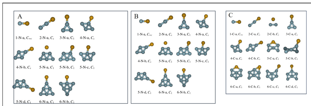
Fig. 3 (A) Optimized structures of neutral Ag n Hg complexes, n \leq 6 . The symmetry point group is indicated. (B) Optimized structures of anionic Ag n Hg complexes, n \leq 6 . The symmetry point group is indicated. (C) Optimized structures of cationic Ag n Hg complexes, n \leq 6 . The symmetry point group is indicated. 45 Reproduced with permission from ref. 45, copyright 2024, Chem. Phys. Lett.
