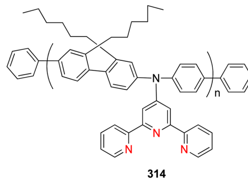
Fig. 18 Chemosensors with triphenylamine-functionalized conjugated polyfluorene.
