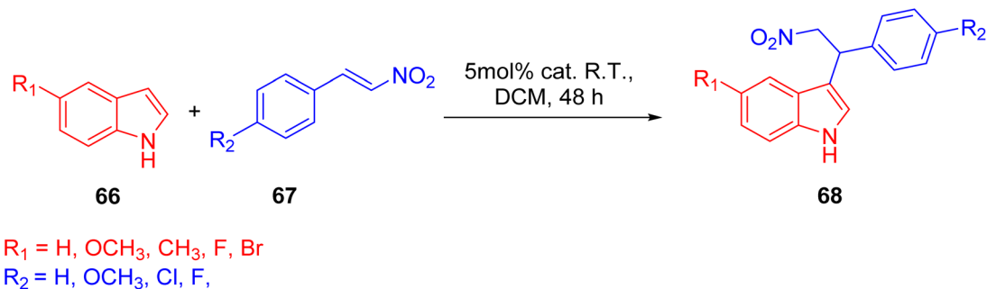
Scheme 20 Friedel–Crafts alkylation of indole and \beta -nitrostyrene catalyzed by compound 66 .
