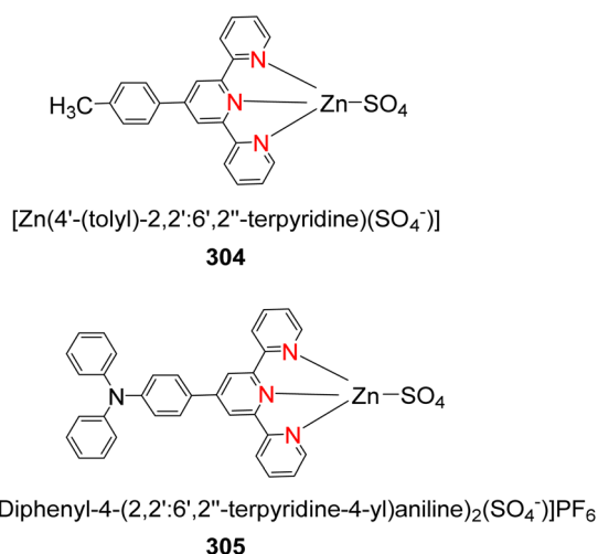
Fig. 12 Complexes acting to photo-degrade methylene blue in wastewater effluents.
