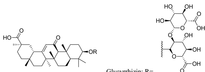
Glycyrrhizin: R=
