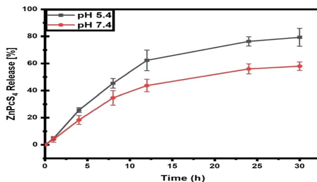
Fig. 1 \text{ZnPcS}_4 release kinetics from the nanoconjugate at both neutral and acidic pHs.
