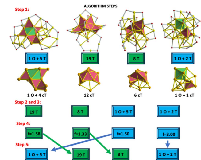
Fig. 3 Implementation of a 5-step algorithm to determine the energy order between isomers of the \text{Au}_{25}(\text{SCH}_3)_{19}^{[0]} cluster. Colour code is the same as that shown in Fig. 2. Upper panel features the number and type of polyhedra found in each total structure (Au–S framework + inner core). The lower panel depicts compact tetrahedra (cT) constituting each inner core. Each step of the algorithm is given in the lower part. Highlighted boxes are used to distinguish between two sets of structures. The last row (step number 5) contains the ordered structures in terms of the corresponding T-factor values.
