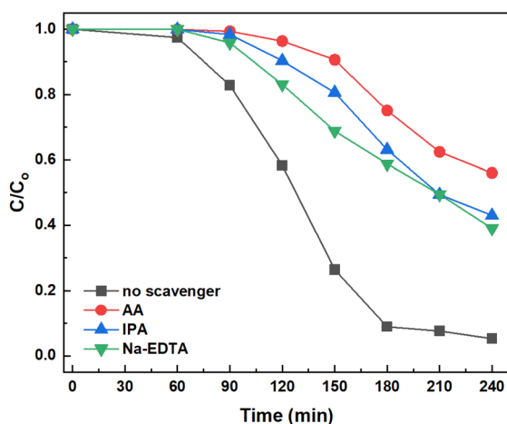
Fig. 17 The influence of \text{O}_2^{\cdot-} , \cdot\text{OH} radicals and photogenerated holes \text{h}^+ on the 2,4-D treatment ( C_0 = 40 ppm, pH = 2.2, 3% \text{AgNPs/g-C}_3\text{N}_4 , 16 mL of 0.1 M Na-EDTA, 16 mL of isopropyl alcohol (IPA) and 1 mL of AA).
