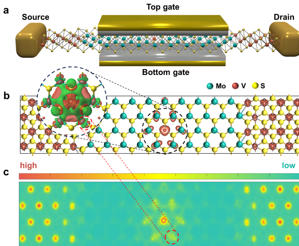
Fig. 2 Schematic diagram of a FET model with \text{VS}_2 electrodes at both ends, V- \text{MoS}_2 channel in the middle ( L_{\text{ch}} = 3.0 nm), and gate electrodes (EOT = 0.5 nm) on top and bottom (a). The real-space DOS at -0.2 eV (b) and corresponding 2D plot (c) are shown with zero source-drain bias applied. The inset in (b) represents the differential charge density at the V-doped site.
