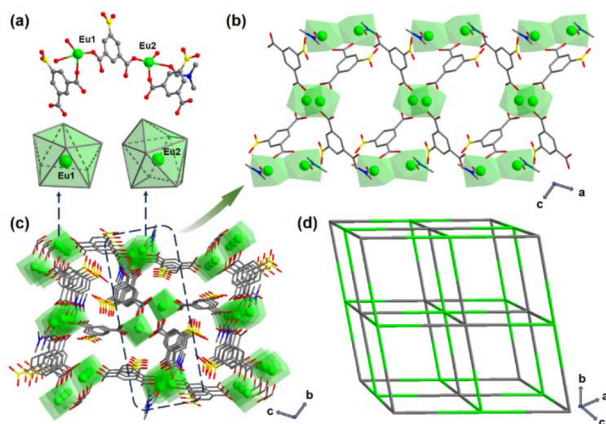
Fig. 1 (a) Minimum asymmetric unit of 7 and coordination configuration of the \text{Eu}^{3+} ions. (b) Connection of binuclear \text{Eu}_2 units and BIPA ^{2-} in the ac plane. (c) Three-dimensional framework of 7 in the bc plane. (d) Simplified pcu topological configuration of 7. Atoms: Eu (green), C (gray), O (red), N (blue), B (yellow); H atoms are omitted for simplification.
