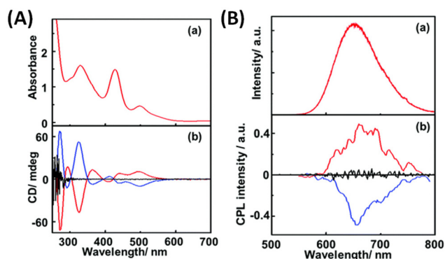
Fig. 3 (A) Absorption (a) and CD spectra (b) of R - (red lines), S - (blue line) and \text{rac-Ag}_{29}(\text{DHLLA})_{12} NCs (black line) and (B) emission (a) and CPL spectra (b) of R - (red lines), S - (blue line) and \text{rac-NCs} (black line). (Reproduced from ref. 41 with permission from the Royal Society of Chemistry, Copyright 2017). DHLLA is \alpha -dihydroxyliipoic acid.
