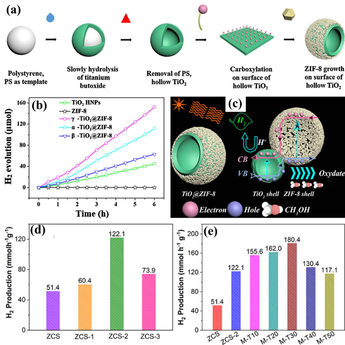
Fig. 18 (a) Diagram showing the incorporation of double-shell TiO 2 /ZIF-8 hollow nanoparticles. (b) The photocatalytic ability for generating the HER of TiO 2 HNPs, ZIF-8, and \alpha - \beta -/ \gamma -TiO 2 /ZIF-8. (c) The operation of the HER over TiO 2 /ZIF-8. Adapted from ref. 389. Copyright © 2019, Elsevier, (d) HER of ZCS composites. (e) ZCS-2, M-TiO 2 , and varied proportions of ZCS-2/M-TiO 2 mixtures. Adapted from ref. 390. Copyright © 2021, Elsevier.
