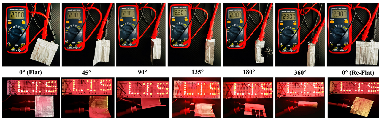
Fig. 6 Upper row: digital pictures of the OCV for the pouch cell consisting of the g-C 3 N 4 -Mx/S cathode at different folding angles. Bottom row: pictures of LEDs lightening up by a pouch cell at different folding angles demonstrating the excellent flexible feature of the developed pouch cell.
