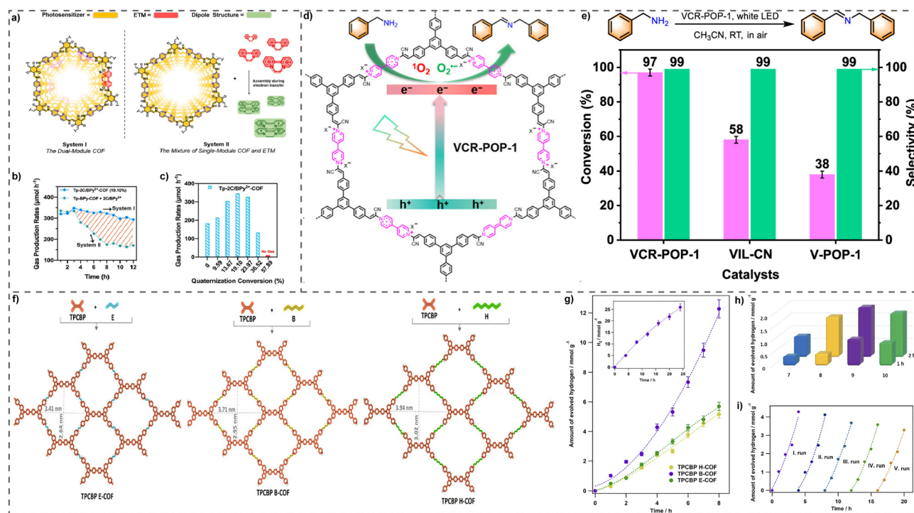
Fig. 11 (a) Schematic diagram of the dual-module COF (System I) and the mixture of single-module COF with unembedded ETM (System II). (b) The hydrogen evolution test of the integrated Tp-2C/Py 2+ -COF (19.10%) and the bare Tp-BPy-COF mixed with additional 2C/Py 2+ used as an ETM under visible-light irradiation. The orange integral area roughly reflects the hydrogen evolution difference between the two photocatalytic systems. (c) HERs of Tp-2C/Py 2+ -COF (10 mg) with different quaternization conversions. Reproduced with permission from ref. 107. Copyright 2022 Wiley-VCH. (d) Schematic representation of photocatalytic oxidative coupling of benzylamine through VCR-POP-1. (e) Photocatalytic performance in white-light-driven photocatalytic oxidative coupling of benzylamine into imine over different catalysts VCR-POP-1, VIL-CN, and V-POP-1. Reproduced with permission from ref. 110. Copyright 2022, American Chemical Society. (f) Schematic representation of TPCBP X-COF [X = ethyl (E), butyl (B), and hexyl (H)] structures. (g) Photocatalytic hydrogen evolution activities of TPCBP X-COFs. (h) pH effect of TEOA. (i) Photocatalytic stability test of TPCBP X-COFs. Reproduced with permission from ref. 108. Copyright 2022, American Chemical Society.
