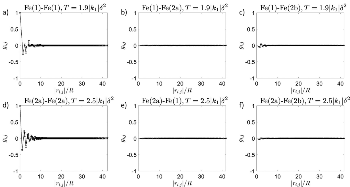
Fig. 8 Two-point spin state correlation function as a function of separation |r_{i,j}| calculated for the simulation depicted in Fig. 3c. (a)–(c) At T = 1.9|k_1|\delta^2 in the \gamma_{HS} = 1/6 plateau. (d)–(f) At T = 2.5|k_1|\delta^2 in the \gamma_{HS} = 5/6 plateau. Correlations between (a) Fe1 sites, (b) Fe1 and Fe2a sites, (c) Fe1 and Fe2b sites, (d) Fe2a sites, (e) Fe2a and Fe1 sites, (f) Fe2a and Fe2b sites. For short distances the correlation between Fe1 sites at T = 1.9|k_1|\delta^2 are weak, and decay rapidly to zero as the distance increases. Similarly, the correlations between Fe2a at T = 2.5|k_1|\delta^2 are weak and decay rapidly to zero as the distance increases. All other correlations are essentially zero. In this figure \Delta\bar{H} = 10.35|k_1|\delta^2 , \delta H_1 = 9.05|k_1|\delta^2 , \delta H_2 = 3.6|k_1|\delta^2 , k_1 > 0 , k_2 = 0.48|k_1| , k_3 = -0.23|k_1| , k_4 = 0|k_1| , k_5 = 0.09|k_1| , and \Delta S = 4\ln(5)k_B .
