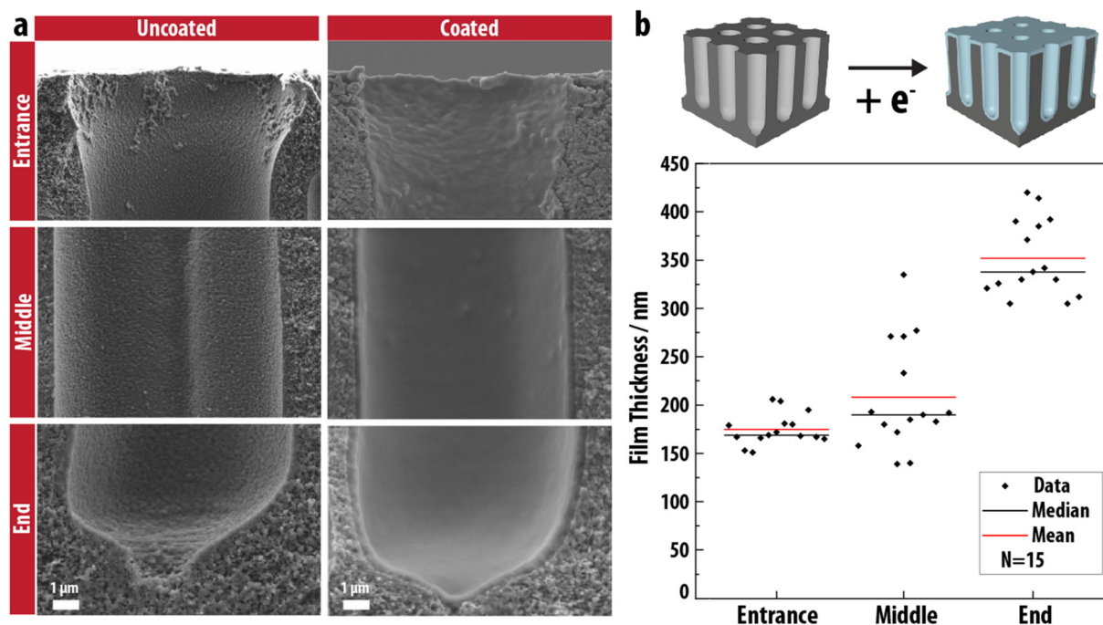
Fig. 2 (a) Cross-sectional SEM images at different locations along an uncoated (left) and a coated (right) 80 μm long pore of a 3-D carbon electrode. (b) Distribution of EPoN-derived PEG coating thickness measured at the three different locations of 15 pores within the 3-D carbon.
