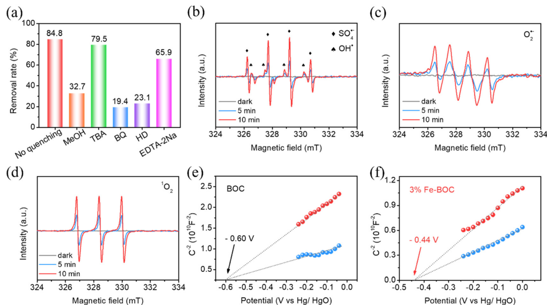
Fig. 7 Scavenging experiment of the active species (a), ESR spin-trapping spectra for the detection of (b) \text{OH}^\bullet and \text{SO}_4^{\bullet-} , (c) \text{O}_2^{\bullet-} and (d) ^1\text{O}_2 , and Mott-Schottky plots of (e) BOC and (f) 3% Fe-BOC.
