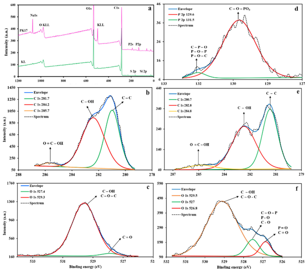
Fig. 7 XPS broad spectra (a), C 1s and O 1s spectra of KL (b and c), C 1s and O 1s, and P 2p spectra of PK17 (d-f).
